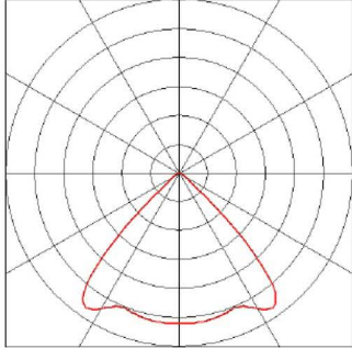
Optic 1: Symmetrical 90x90° beam.
